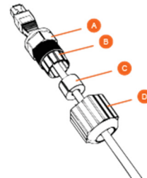
Figure 5 – RJ-45 cable and cable gland assembly
